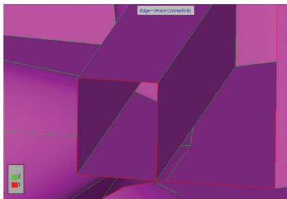
This example illustrates a typical ‘impossible shape’. A hole in the casting overlaps the outside wall.
